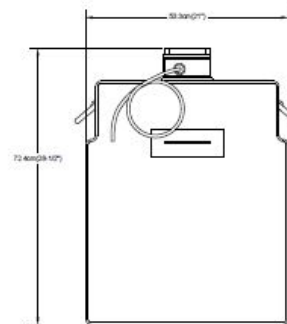
REAR VIEW OF HEATED GFEW ASSEMBLY
