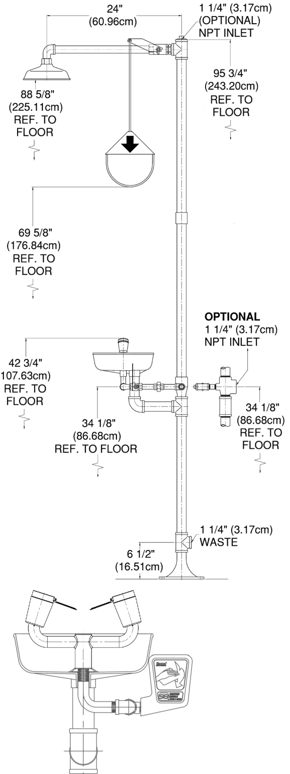
FRONT VIEW (EYEWASH)
